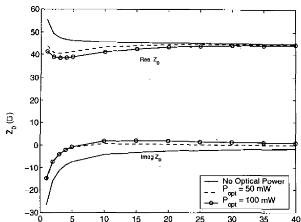
Fig. 5 Complex characteristic impedance of the TWPD for different levels of optical power.
