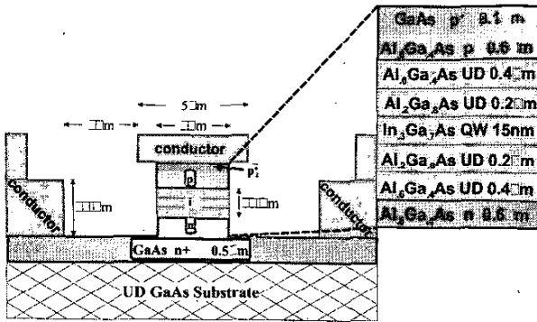
Fig. 1 Cross-section of the TWPD taken from [4].
