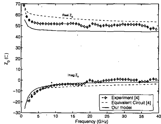
Fig. 4 Complex characteristic impedance of the TWPD for zero optical power.
